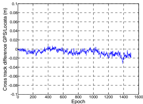
Figure 12. Circuit 1 cross-track difference GPS & Locata .
