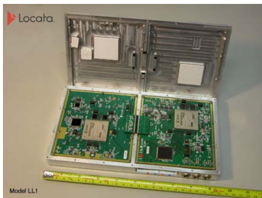
Figure 2. LocataLite (transceiver) hardware.
