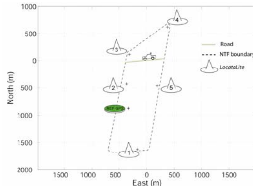
Figure 7. LocataNet setup for kinematic test.
