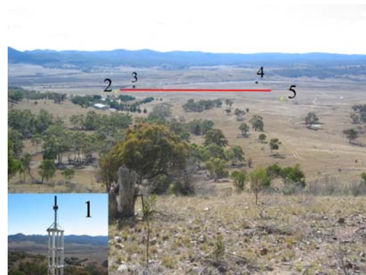
Figure 6. View of NTF and test area from LocataLite 1. The road is marked in red.
