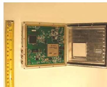
Figure 3. Locata Receiver hardware.
