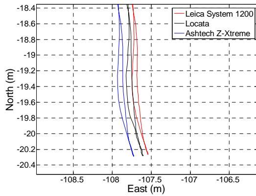
Figure 10. Circuit 1 GPS and Locata position trajectories from top to bottom: full circuit, start/end location, turn at East end, and 'zoomed' East end turn.
