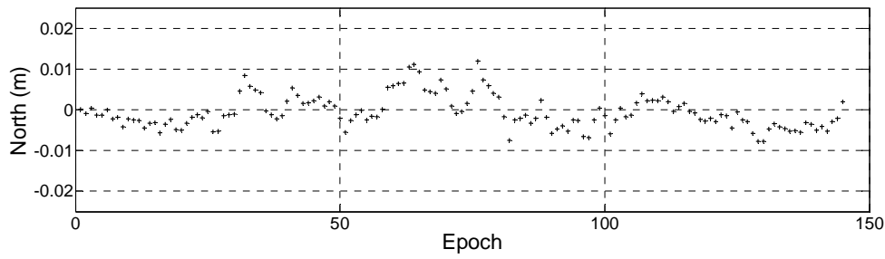
Mean static East and North time series: Locata (top), GPS (bottom)
