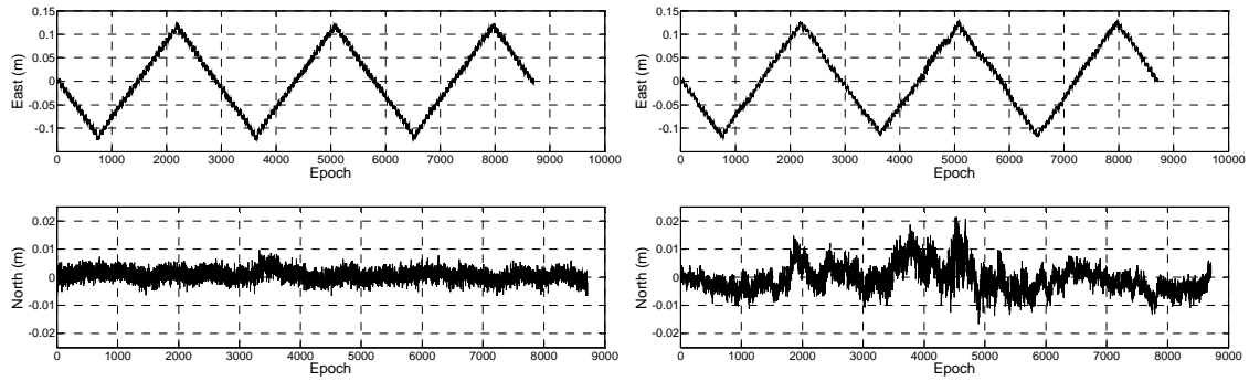
Figure 7 East and North time series: Locata (left), GPS (right)
