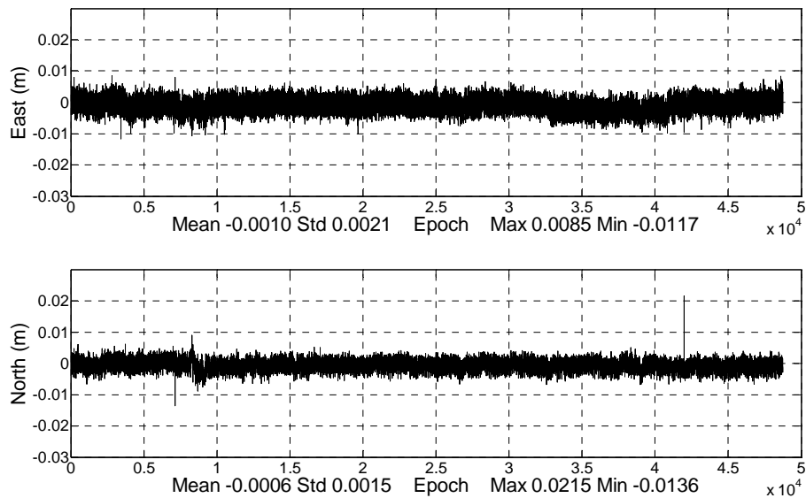
Figure 4 East and North error for long term (13.5 hour) static positioning test.
