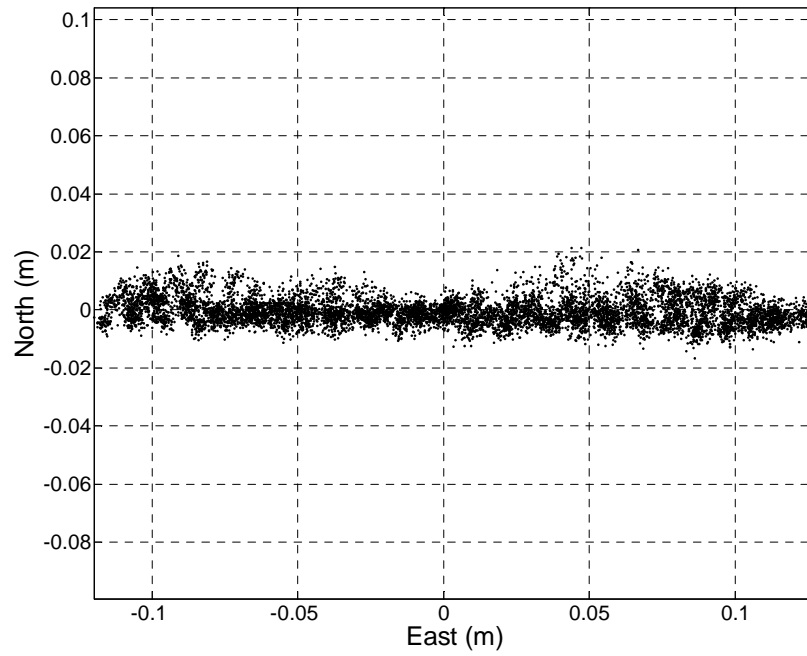
Horizontal trajectory: Locata (top), GPS (bottom)
