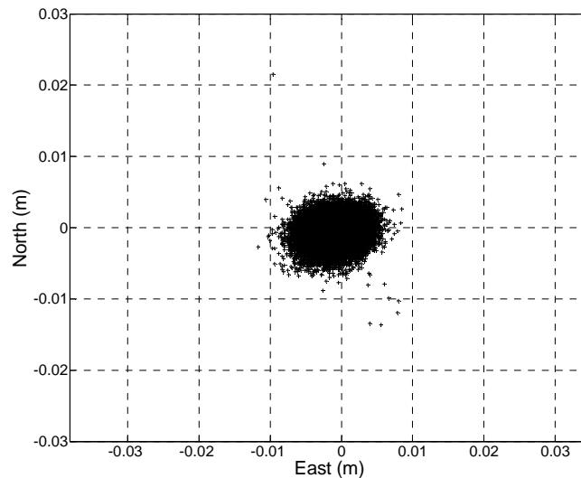
Figure 3 Horizontal error scatter plot for long term (13.5 hour) static positioning test.
