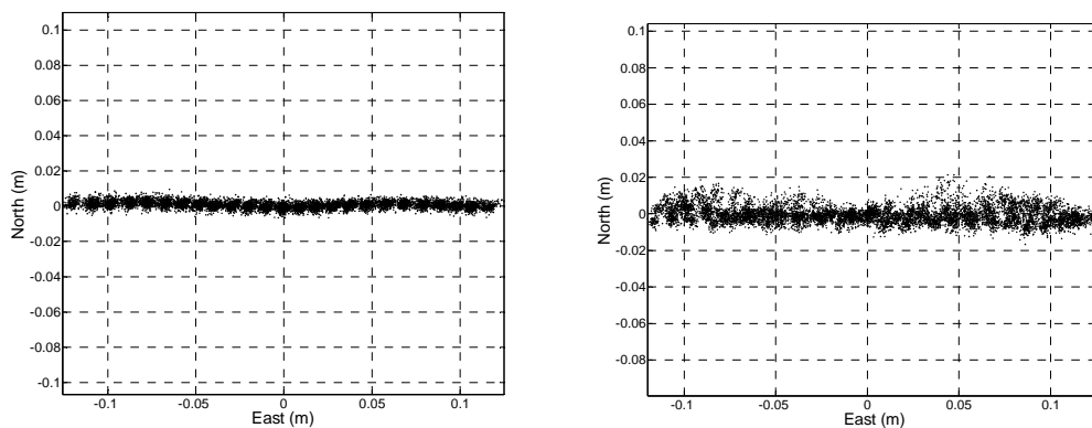
Figure 6 Horizontal trajectory: Locata (left), GPS (right)
