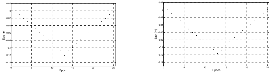
Figure 10 Mean static East 1 st 24 moves: Locata (left), GPS (right)
