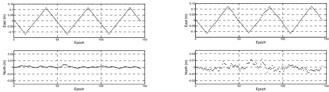
Figure 9 Mean static East and North time series: Locata (left), GPS (right)
