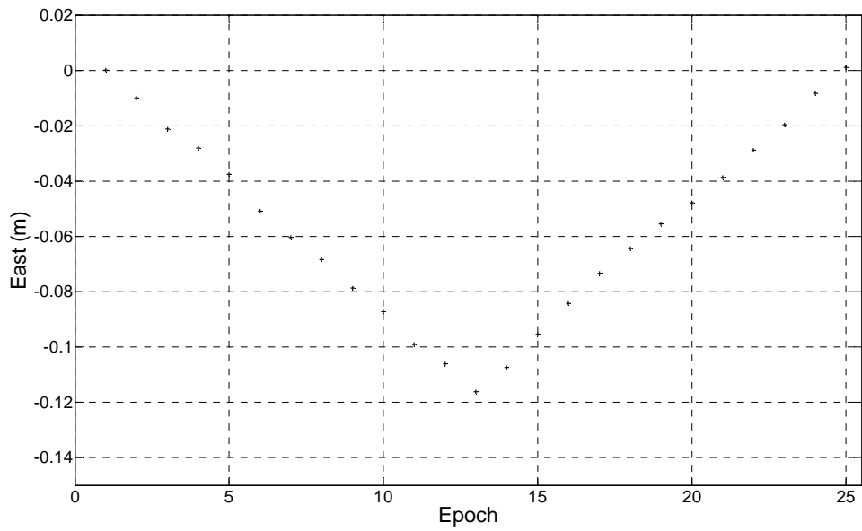
Mean static East 1 st 24 moves: Locata (top), GPS (bottom)
