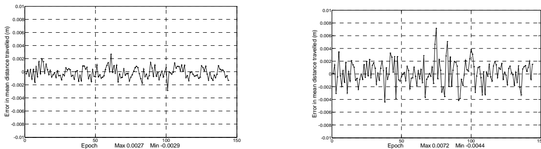
Figure 12 Error in distance travelled for each 1cm move (computed from mean position values): Locata (left), GPS (right)
