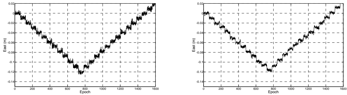
Figure 8 East time series, 1 st 1600 epochs: Locata (left), GPS (right)
