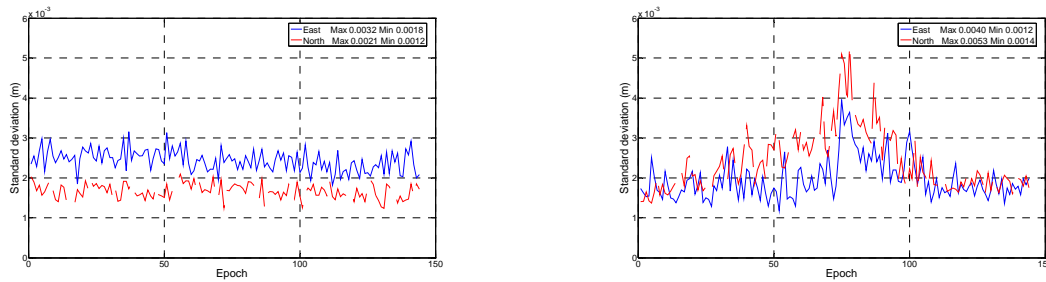
Figure 11 Standard deviation of static East and North: Locata (left), GPS (right)
