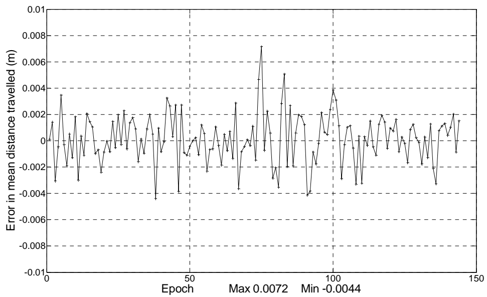
Error in distance travelled for each 1cm move (computed from mean position values): Locata (top), GPS (bottom)
